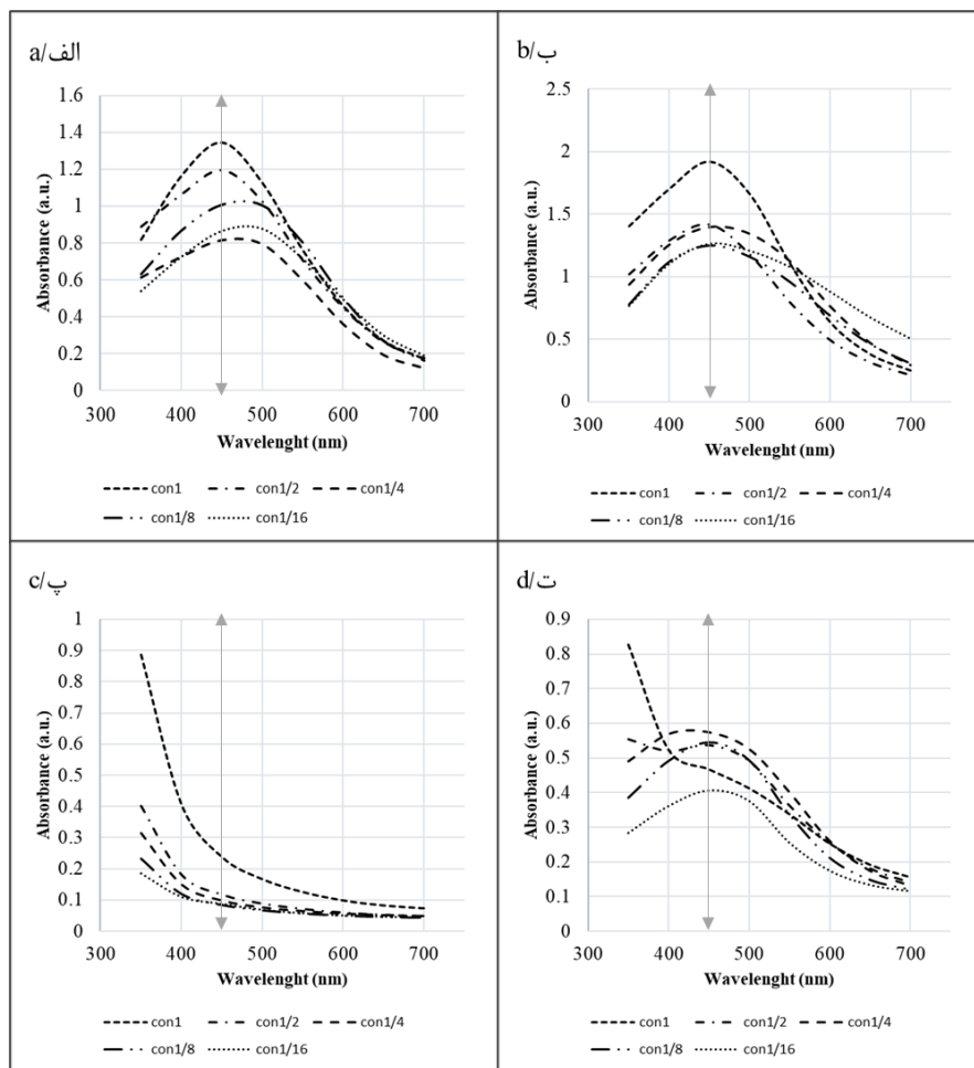
Fig. 8. UV/Vis spectroscopy of silver nanoparticles with diluter extract, a, b, c and d, respectively different concentration of aqueous plant extract and 1 mM AgNO 3 under whit, blue, red and green light.
