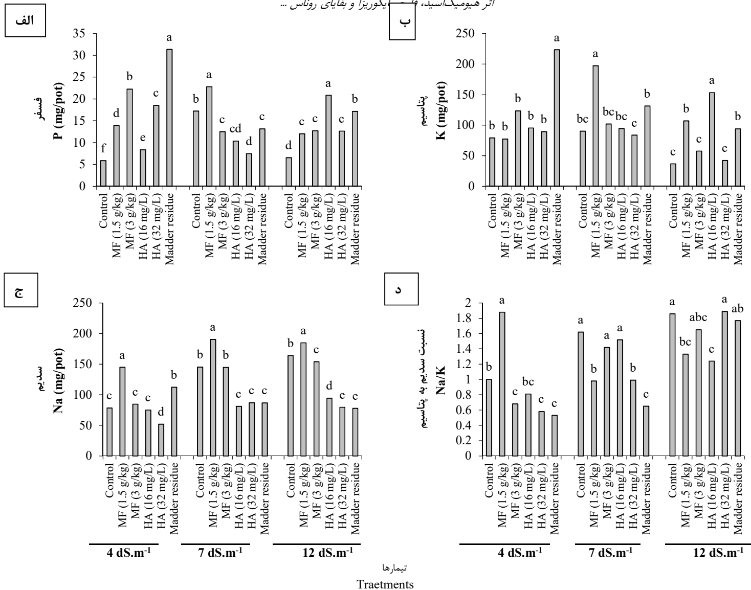
Fig. 1. The interaction of organic and biological fertilizers and salt stress on uptake of P (a), K (b), Na (c) and Na:K ratio (d) of evening primrose ( O. biennis L.) (MF: Mycorrhiza Fungi and HA: Humic Acid) † Means with different letters are significantly different ( p \leq 0.05 ) based on Duncan test.
