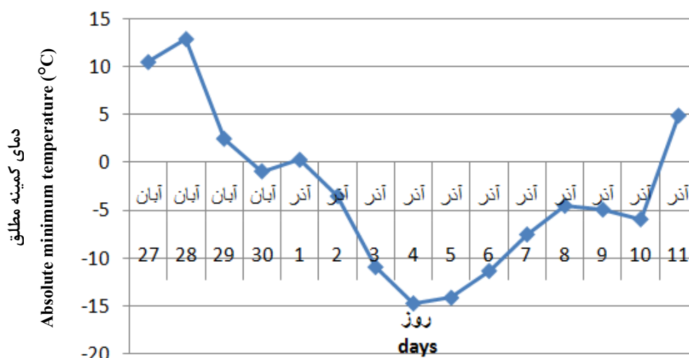
Fig. 1. Trend of absolute daily minimum temperature changes at Khondab meteorological station (Nearest meteorological station to vineyard used for this research) from November 17 th , to December 1 th 2016 when occurrence early fall frost.
