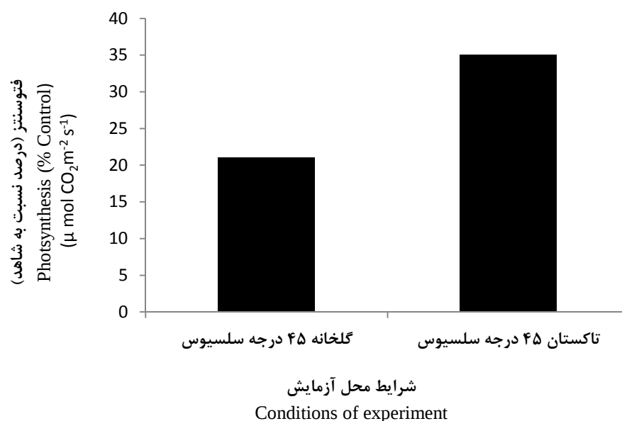
Fig. 1. Leaf photosynthesis rate for Yaghooti grapevine cultivar under 45^\circ\text{C} heat stress in greenhouse and vineyard in comparison with no heat stress conditions (control).
