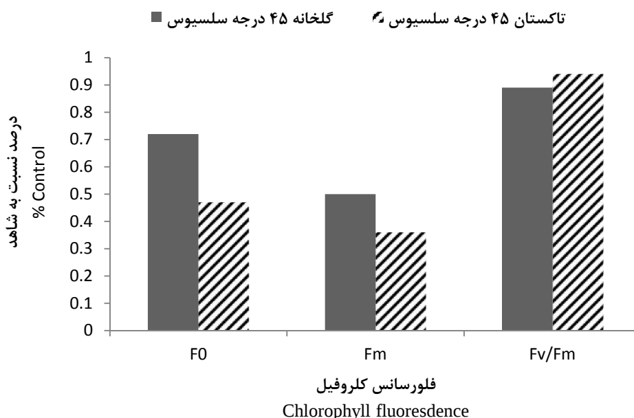
Fig. 3. Chlorophyll fluorescence in Yaghooti grapevine cultivar in comparison with no heat stress (Control). Minimum fluorescence (F0), Maximum fluorescence (Fm), Maximum quantum yield of PSII (Fv/Fm)
